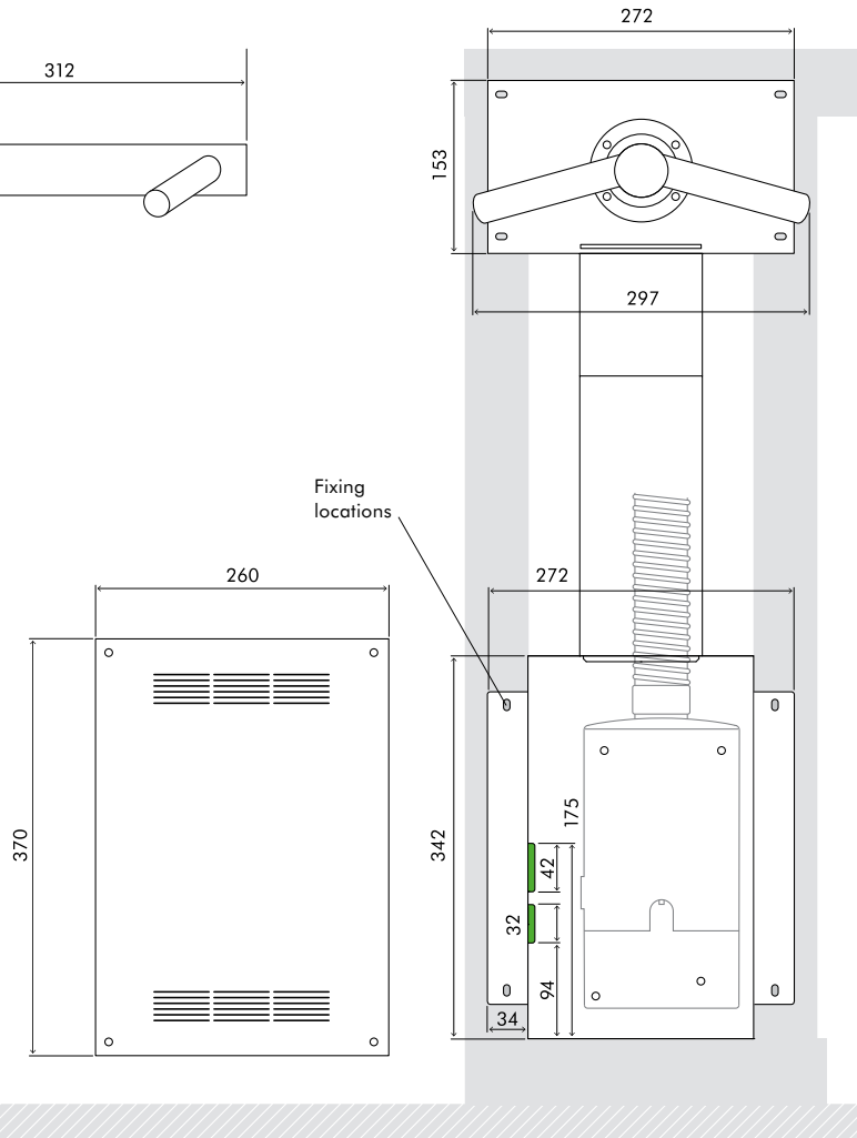
REAR ELEVATION
