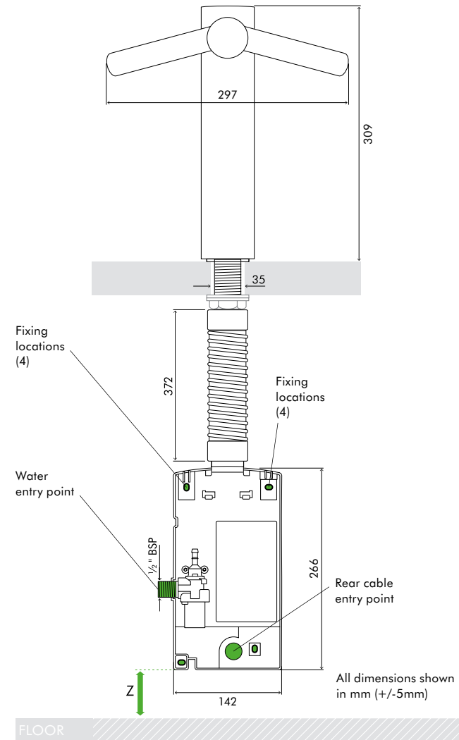
REAR ELEVATION
