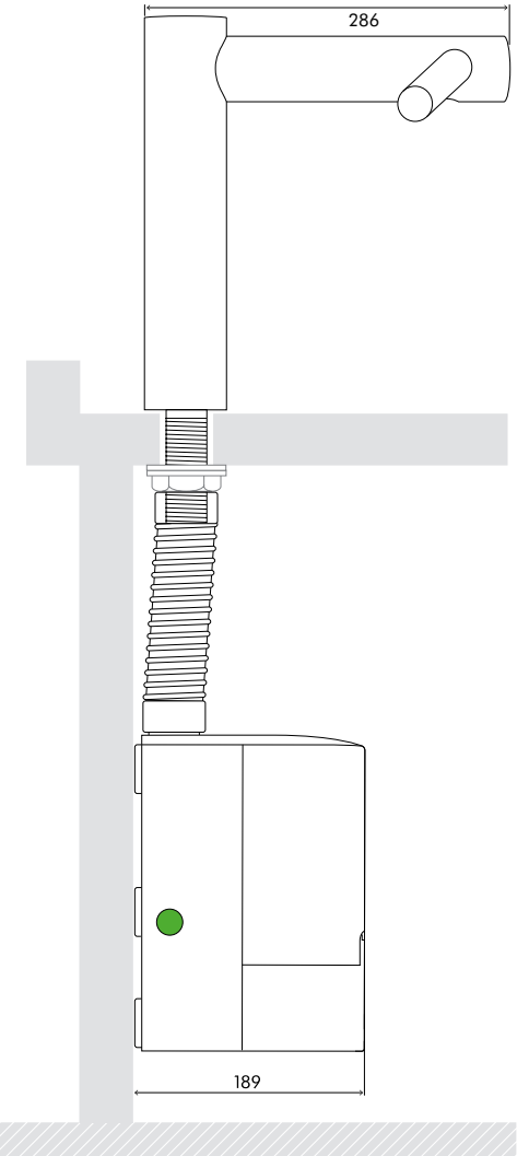
SIDE ELEVATION
