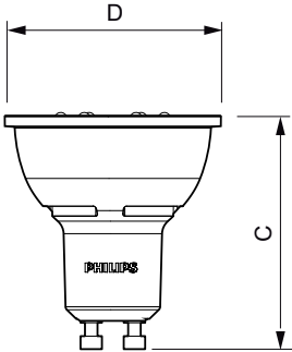
LED 5-50W GU10 830 36D
