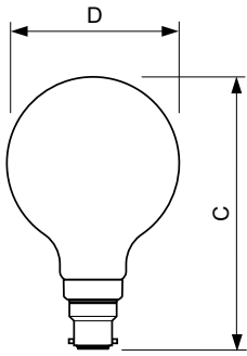
filament G120 7W-48W 620lm 2000K B22 D
