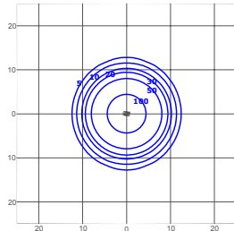
lux STL-A-NM-90-27L-408-+-24-45-WH-DIM Mounting Height: 10m
