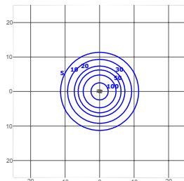
lux STL-A-NM-12-13L-408-+-24-45-WH-DIM Mounting Height: 6m
